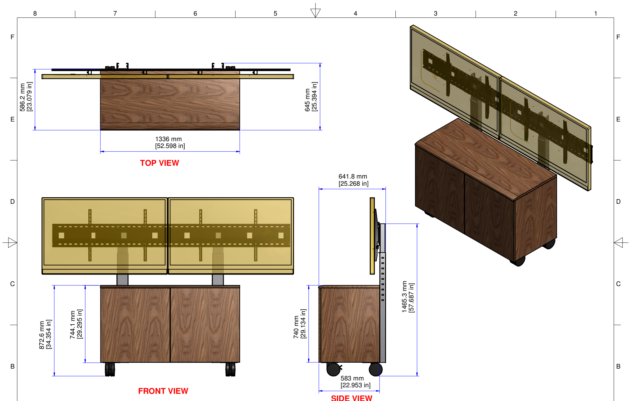
SIDE VIEW
