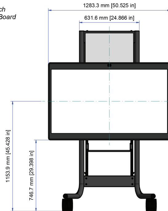
FRONT VIEW - Lowest height
