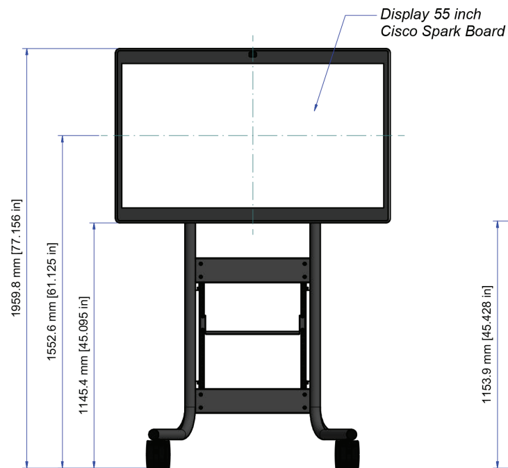
FRONT VIEW - Full height
