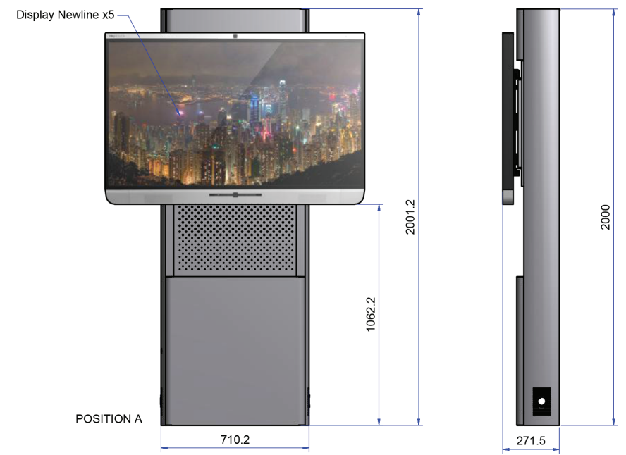
FRONT VIEW - Full height
