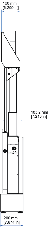
SIDE VIEW POSITION I
