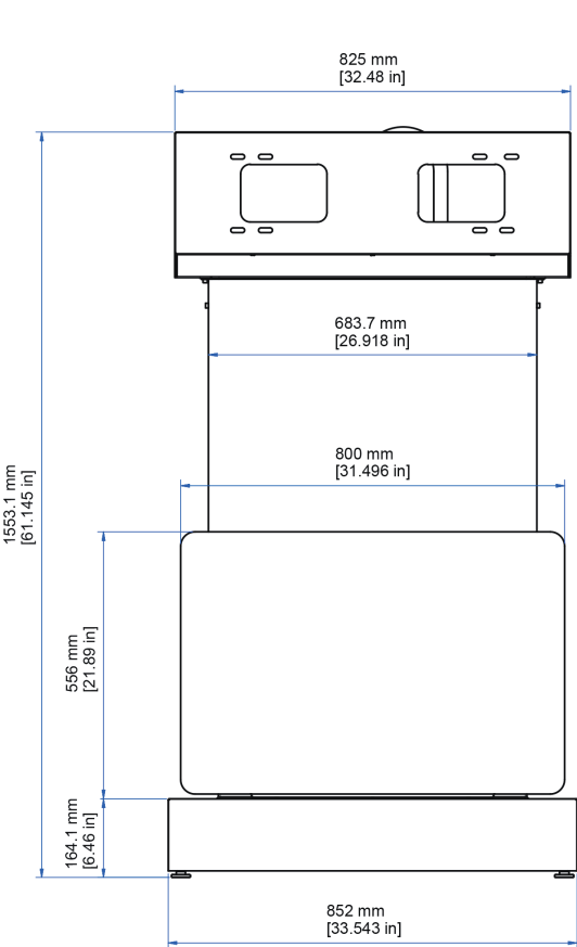
FRONT VIEW POSITION I
