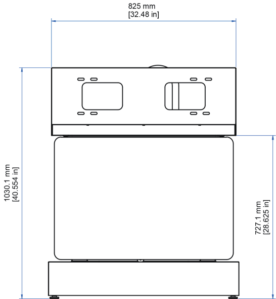
FRONT VIEW POSITION II
