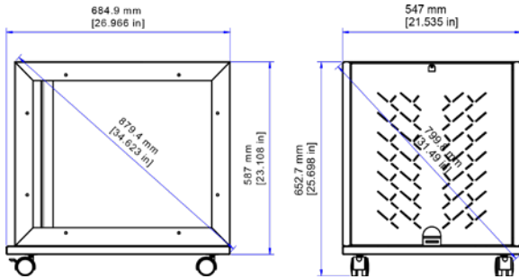
Frame Dimensions
