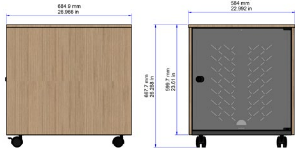
Cabinet Dimensions
