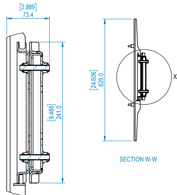
DETAIL X SCALE 1:4
